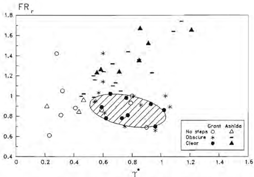
Figure 6: Domain of step formation. Shaded area represents zone of clear steps. Data from Ashida et al (1984) also shown.
