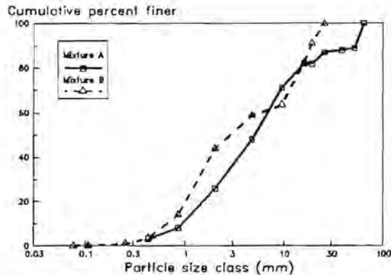
Figure 2: Particle size distributions for the two experimental mixtures.
