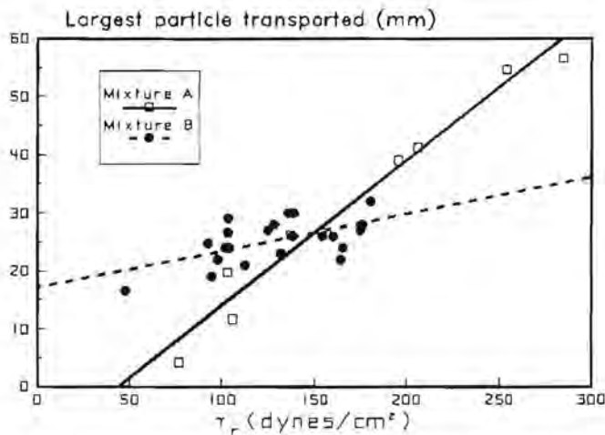
Figure 3: Results from incipient motion experiments for the two mixtures shown in Fig. 2.
