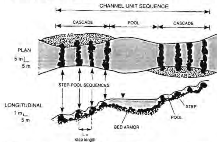
Figure 1: Plan and side view of channel unit and step-pool sequences, showing bed armor and alternate bars (AB).
