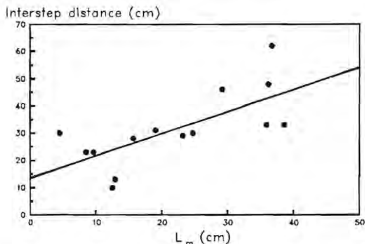
Figure 5: Interstep distance (measured crest-to-crest) as a function of antidune spacing as defined by the wave number L_m = 2\pi v^2/g .
