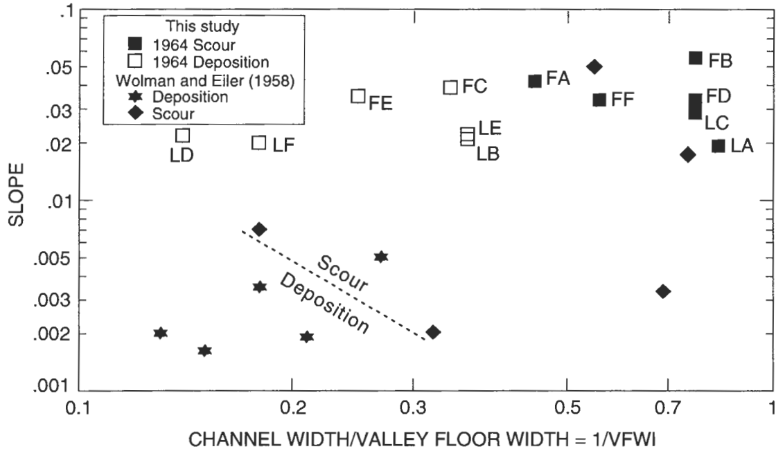
Fig. 9. Patterns of scour and deposition during floods in relation to channel gradient and the ratio of channel width to valley floor width, after Wolman and Eiler [1958]. Shown are Lookout and French Pete Creek reaches and data points for the Connecticut River following the 1955 flood. The dotted line is Wolman and Eiler's [1958] envelope curve (fitted by eye) distinguishing domains of scour and deposition for their data.
