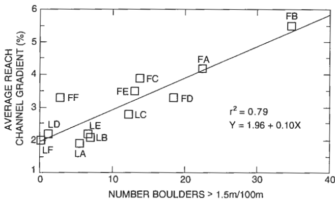
Fig. 8. Relation between average channel gradient and average boulder densities by reach.
