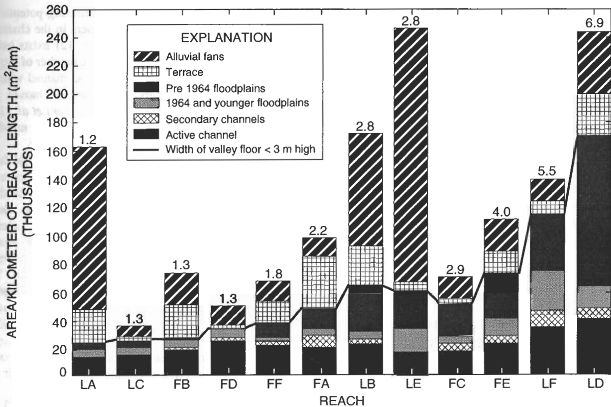
Fig. 6. Distribution of valley floor surfaces by reach for both sites ordered by valley floor width index (shown above bars). Reaches were identified by a two-letter code, where the first letter denoted the site (F = French Pete Creek, L = Lookout Creek) and the second denoted the order of the reach (A = furthest downstream, F = furthest upstream). Vertical axis is the total area by reach in each surface type divided by the reach length.
